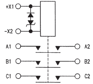
Circuit Configuration 3
